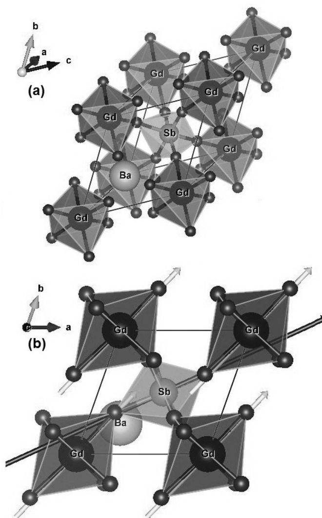
Fig. 2. (a) Characteristic cell and (b) \text{GdO}_6 and \text{SbO}_6 octahedra in the ab -plane for trigonal structure of the \text{Ba}_2\text{GdSbO}_6 double perovskite
