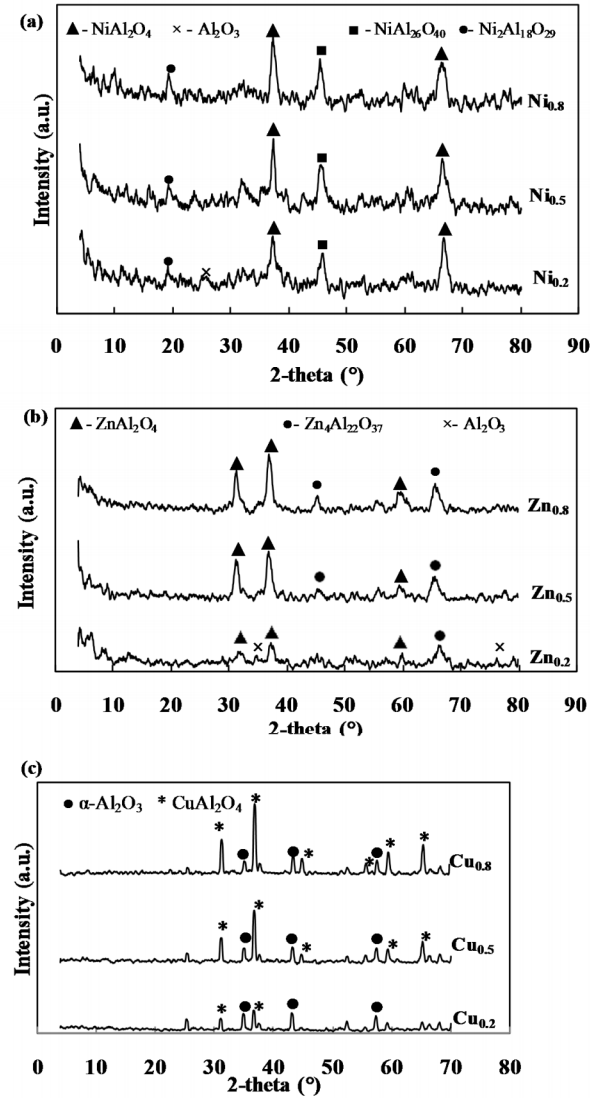
Fig. 1. XRD pattern of metal aluminates with various metal contents (a) nickel, (b) zinc and (c) copper
