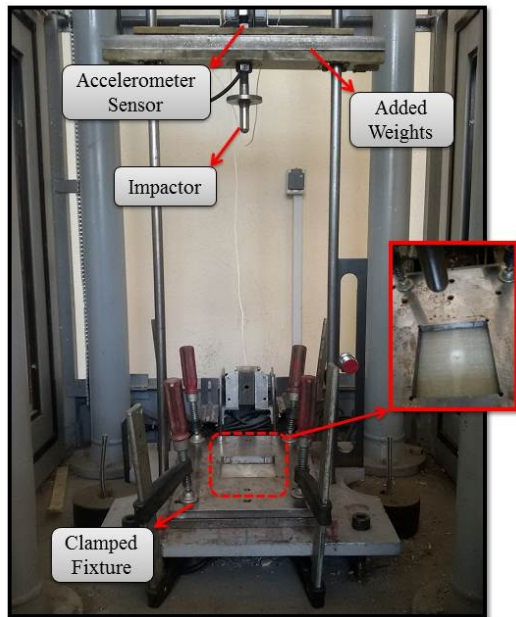
Fig. 2. The LVI test setup.
