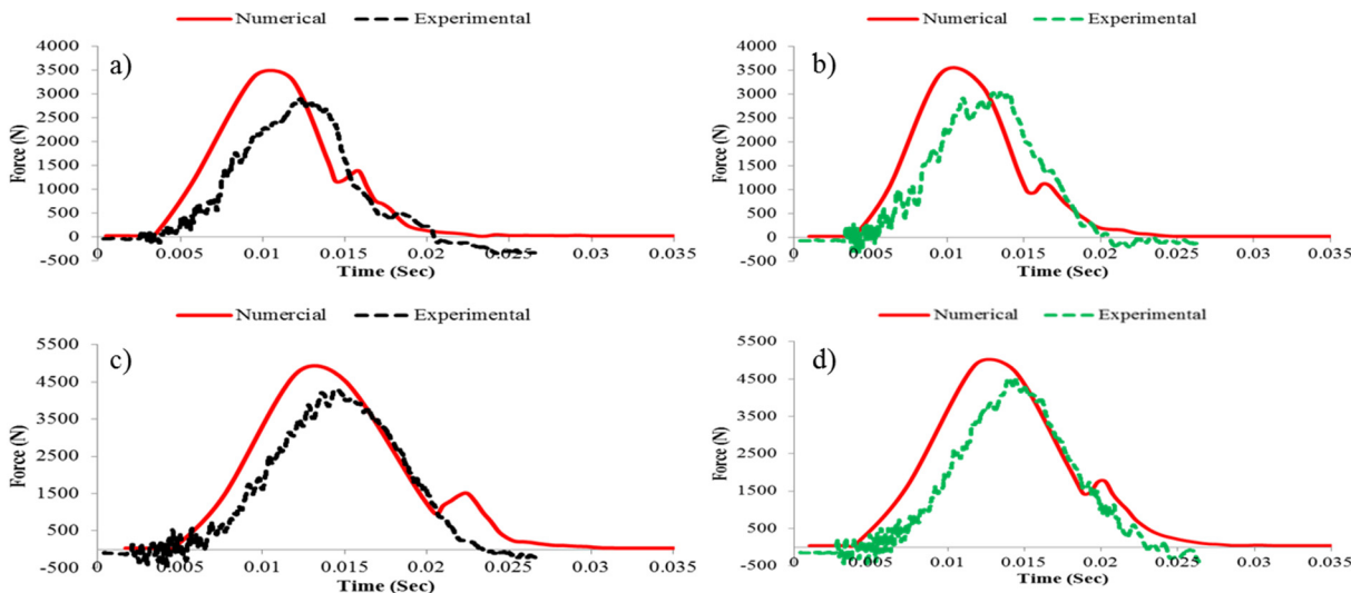
Fig. 9. Comparative force- time response obtained from experimental and numerical investigation for: a and c) pure GFRP subjected to 21 and 30J energy, b and d) incorporated GFRP with 0.3 wt% of SWCNT subjected to 21 and 30J energy.
